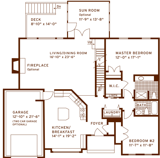
TWO BEDROOM FIRST FLOOR: 1,532 sq. ft. PLUS BASEMENT
